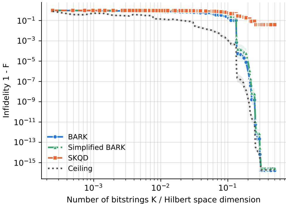
runs per point -- BARK: 42-162, Ceiling: 42-162, SKQD: 42-162, Simplified BARK: 42-162
