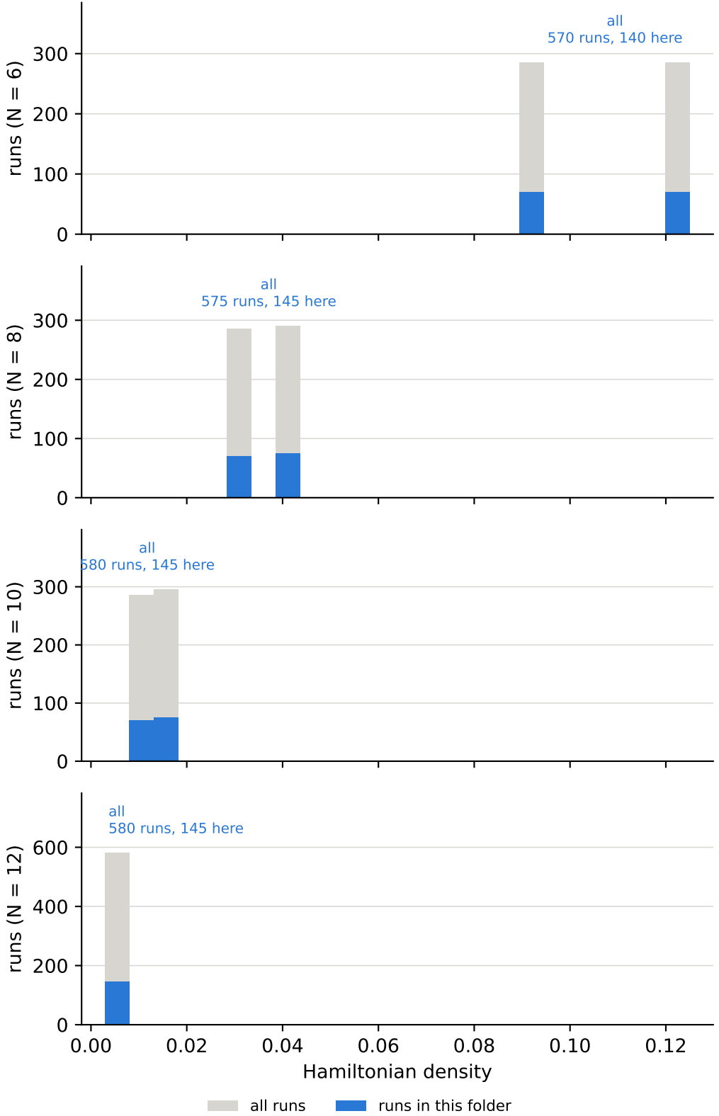
Hamiltonian density over all runs, and the cuts behind the bins field B_z = high, Hamiltonian density = all
