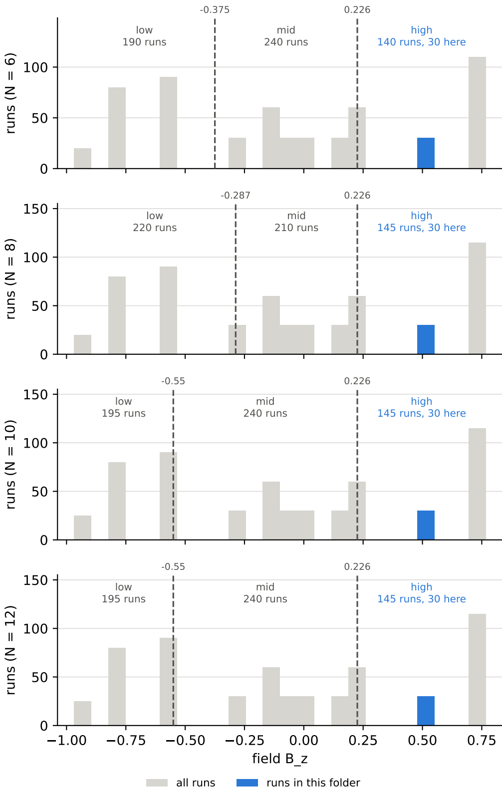
field B z over all runs, and the cuts behind the bins coupling J = mid, field B z = high
