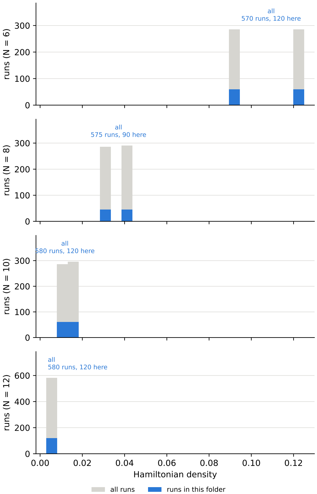
Hamiltonian density over all runs, and the cuts behind the bins coupling J = low, field B_z = mid, Hamiltonian density = all
