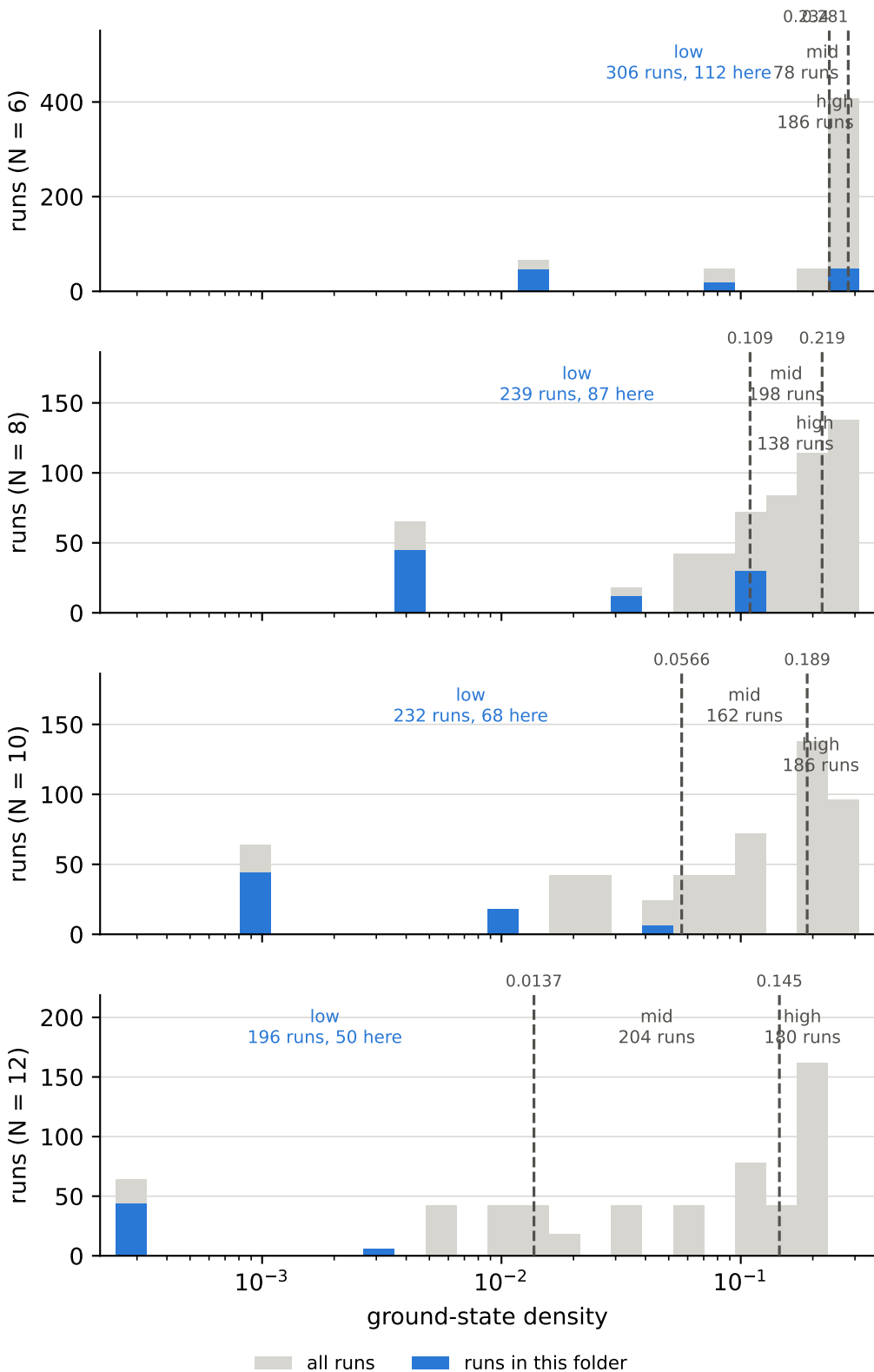
ground-state density over all runs, and the cuts behind the bins coupling J = low, ground-state density = low
