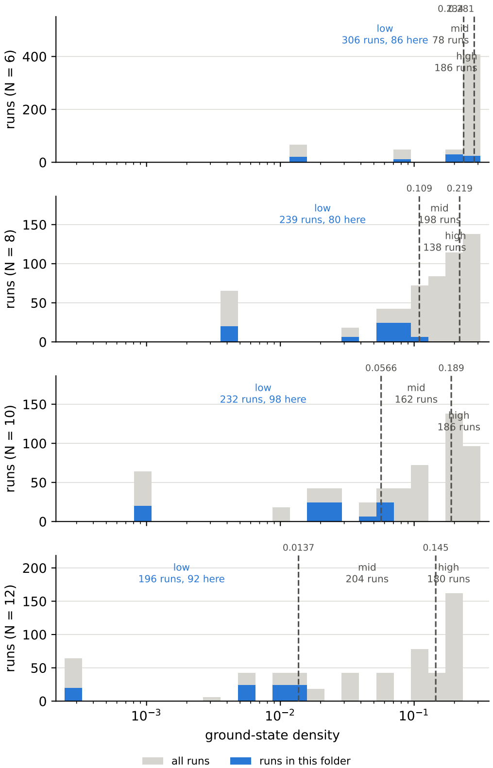
ground-state density over all runs, and the cuts behind the bins coupling J = mid, ground-state density = low
