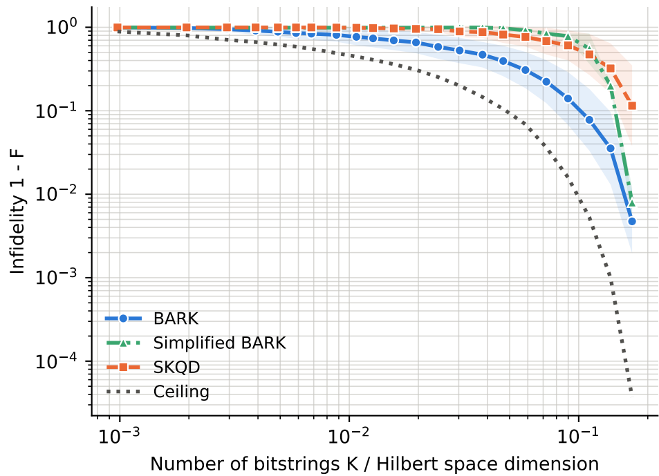
runs per point -- BARK: 24, Ceiling: 24, SKQD: 24, Simplified BARK: 24
