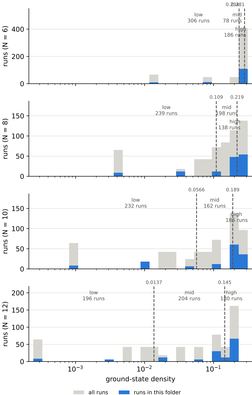
ground-state density over all runs, and the cuts behind the bins anisotropy delta = 0.5
