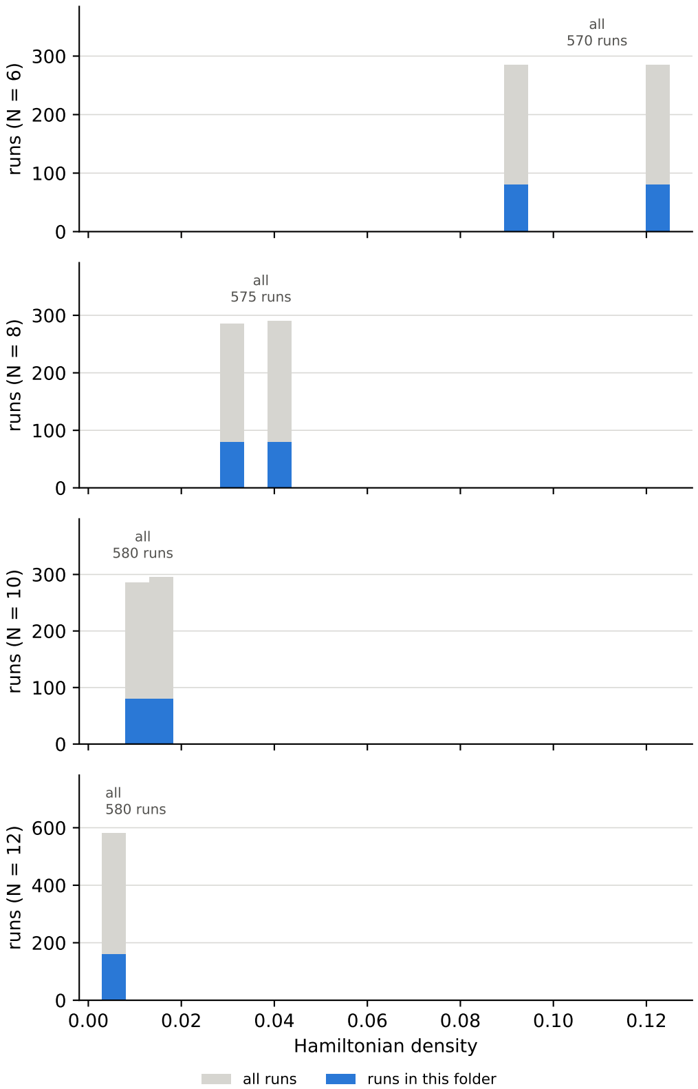
Hamiltonian density over all runs, and the cuts behind the bins anisotropy \Delta = 0
