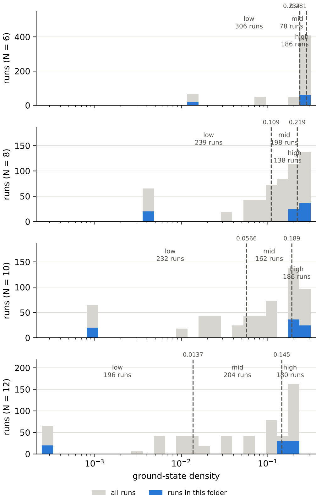
ground-state density over all runs, and the cuts behind the bins anisotropy \Delta = 1
