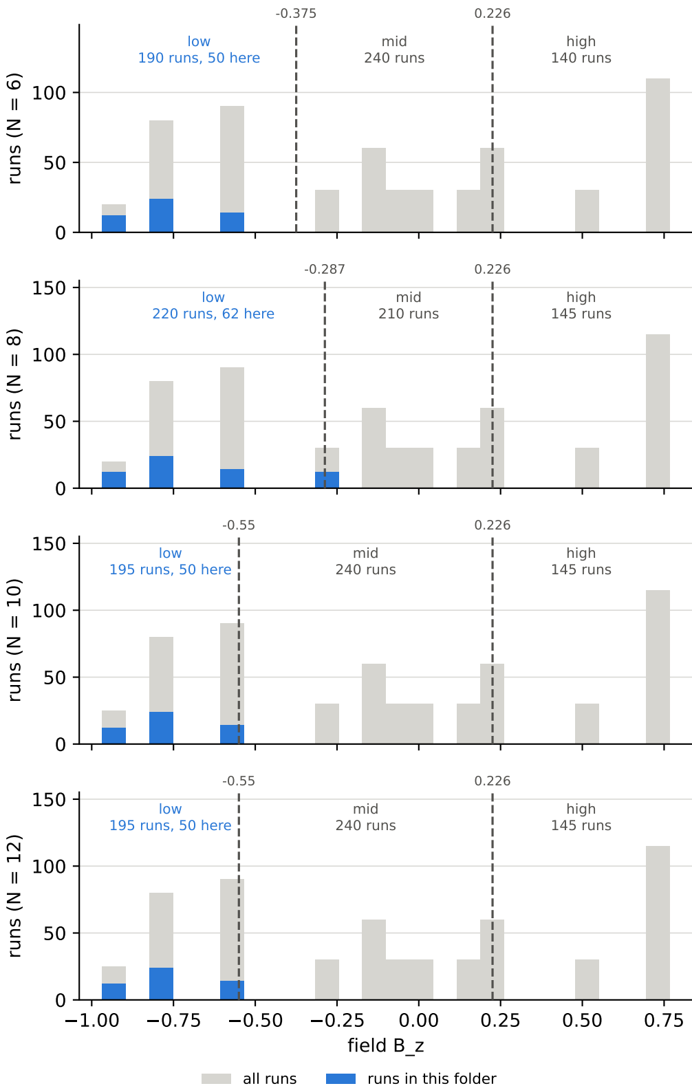
field B_z over all runs, and the cuts behind the bins anisotropy \delta = 0 , field B_z = low
