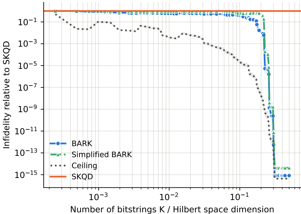
anisotropy \delta = 10 , coupling J = \text{high} (band: standard error)
