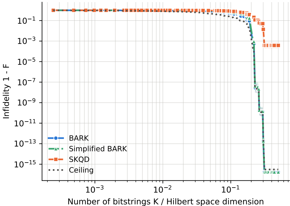
anisotropy delta = 0.5, ground-state density = high (band: standard error)
