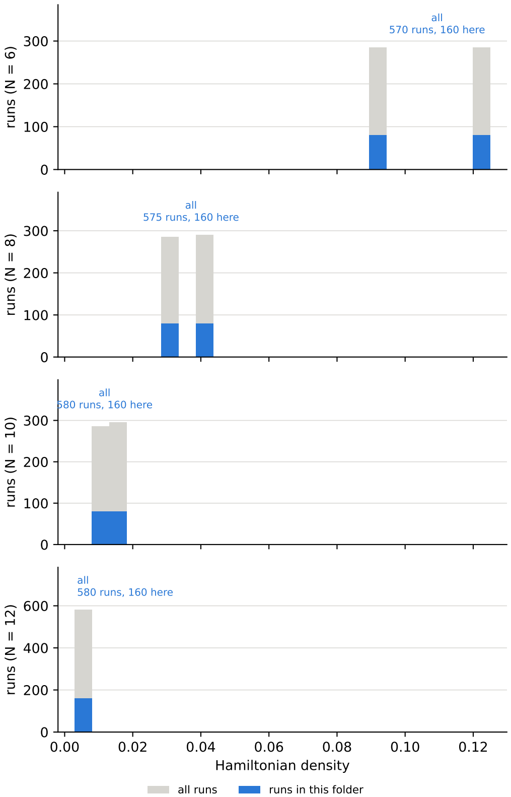
Hamiltonian density over all runs, and the cuts behind the bins anisotropy \Delta = 0 , Hamiltonian density = all
