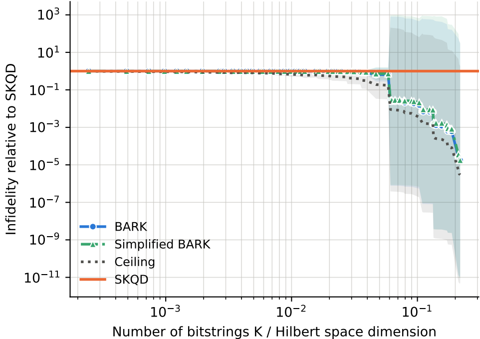
runs per point -- BARK: 14-39, Ceiling: 14-39, SKQD: 14-39, Simplified BARK: 14-39
