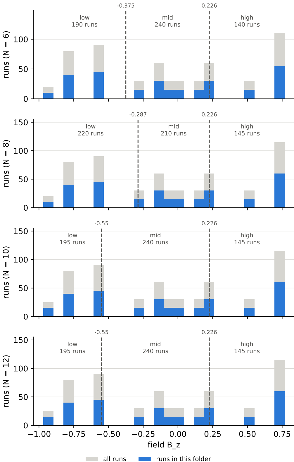
field B z over all runs, and the cuts behind the bins lattice dimension = 2
