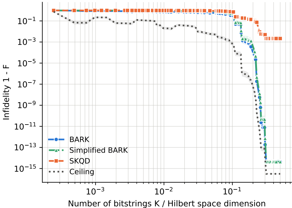
lattice dimension = 2, coupling J = high (band: standard error)
