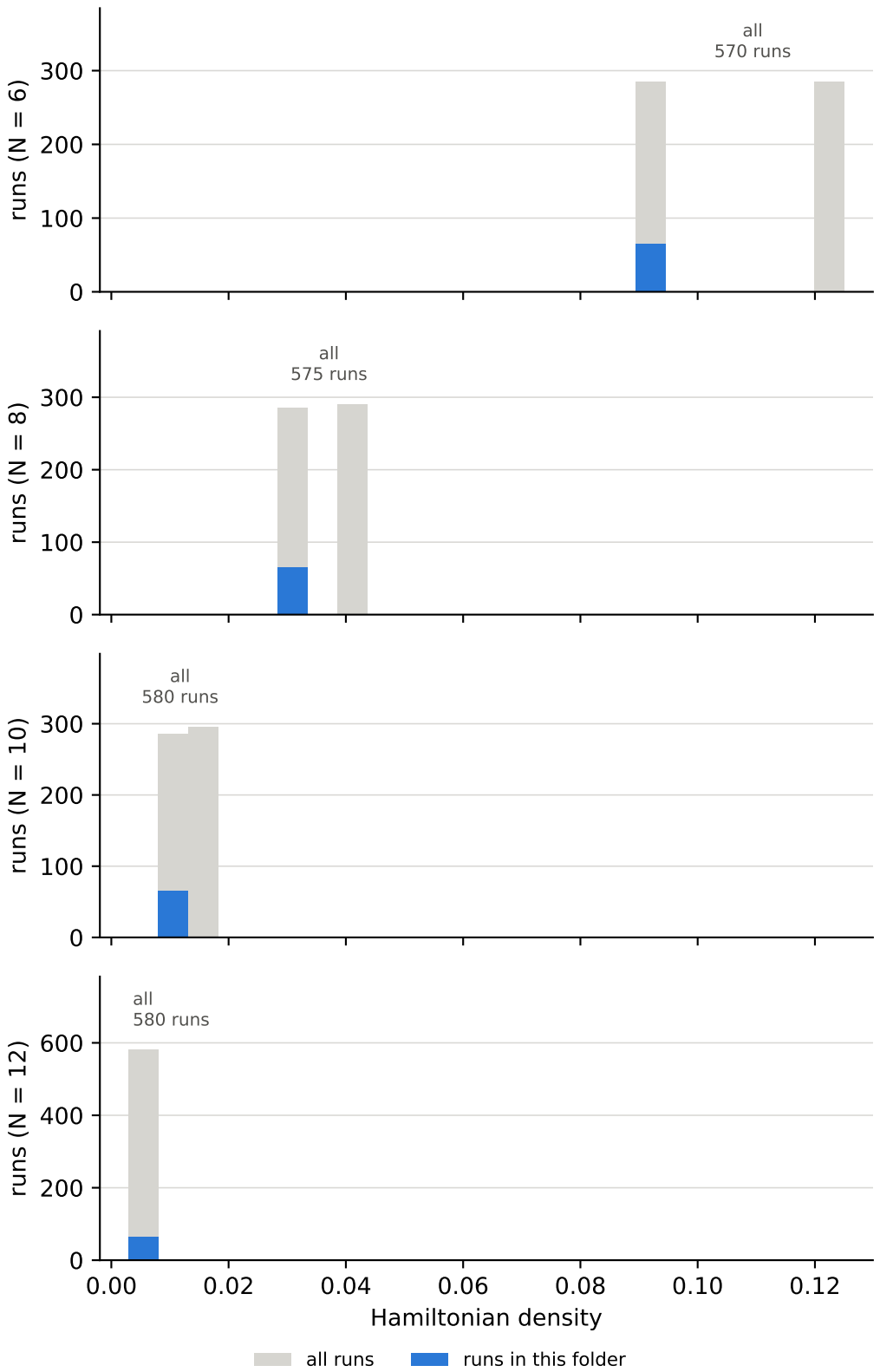
Hamiltonian density over all runs, and the cuts behind the bins lattice dimension = 1, anisotropy delta = 0.5
