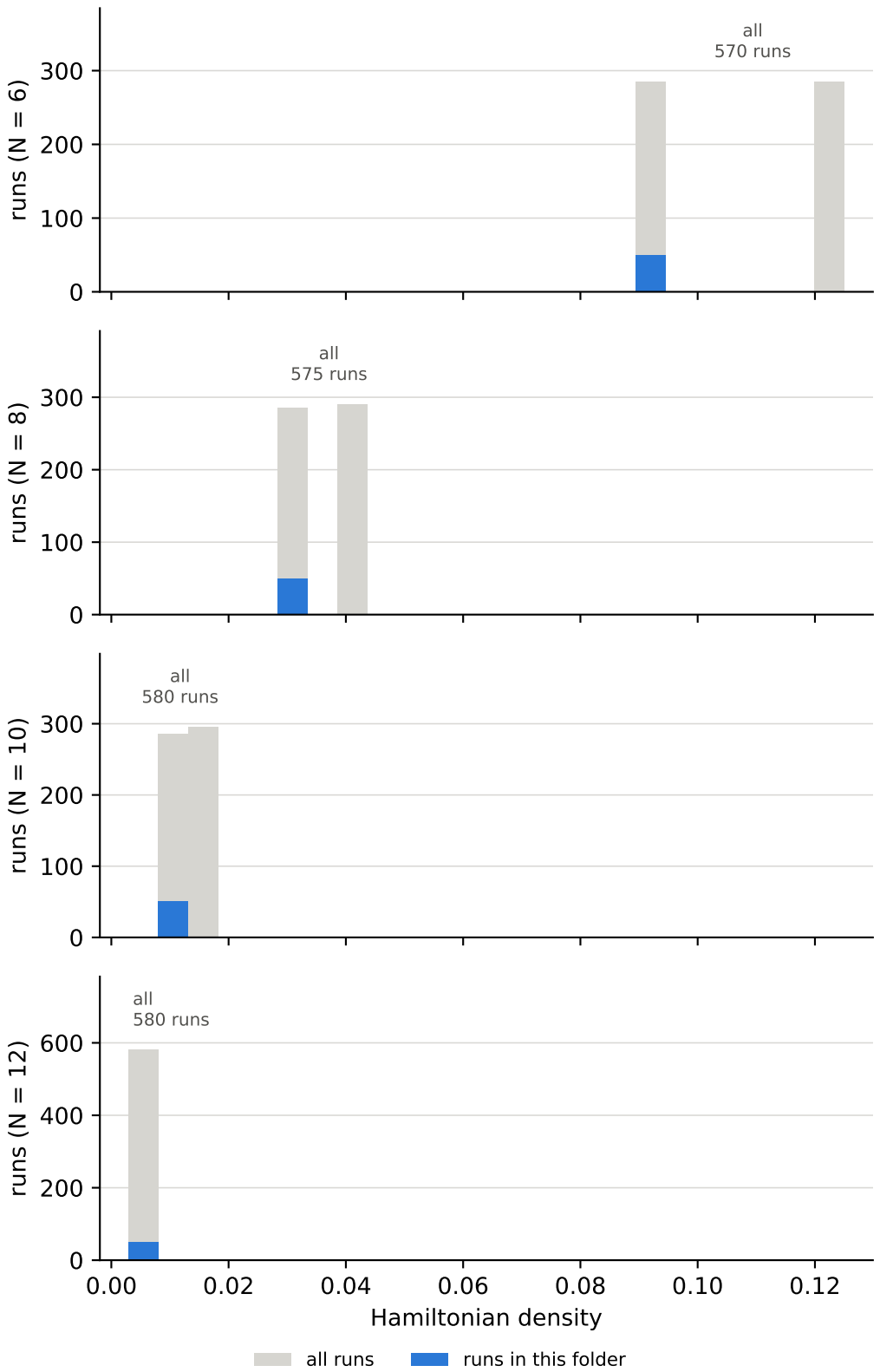
Hamiltonian density over all runs, and the cuts behind the bins lattice dimension = 1, anisotropy \Delta = 10
