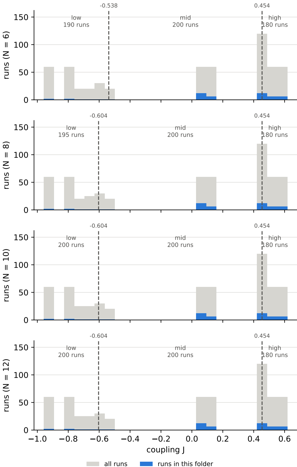
coupling J over all runs, and the cuts behind the bins lattice dimension = 2, anisotropy delta = 10
