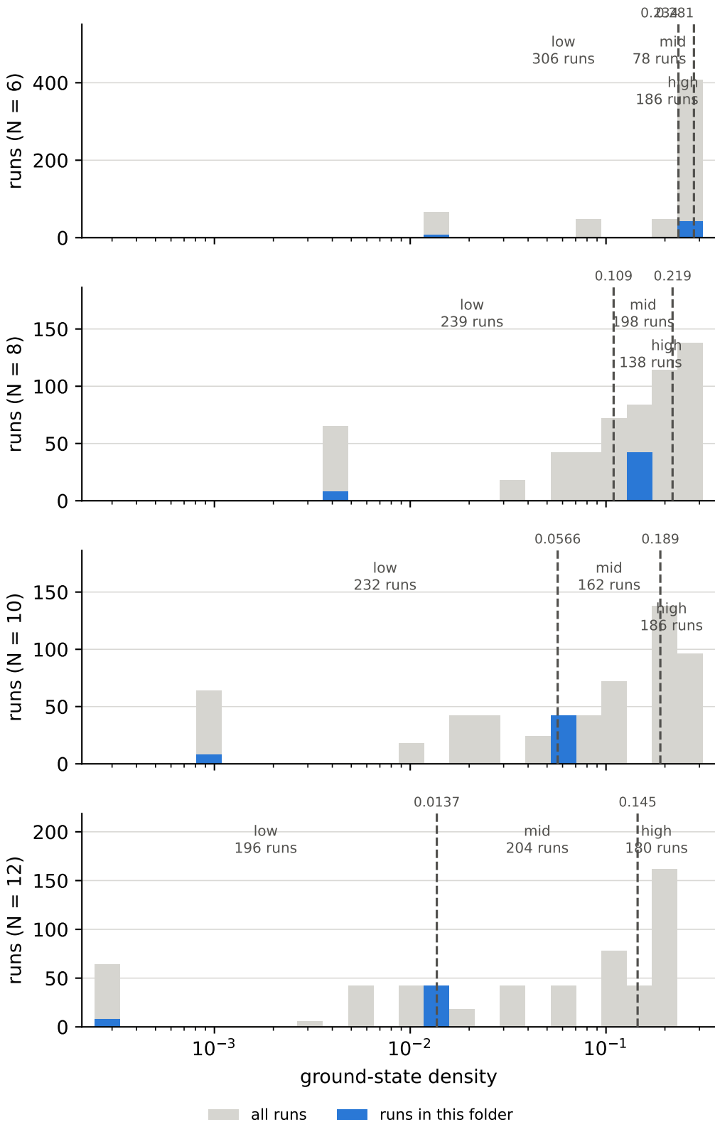
ground-state density over all runs, and the cuts behind the bins lattice dimension = 2, anisotropy \delta = 10
