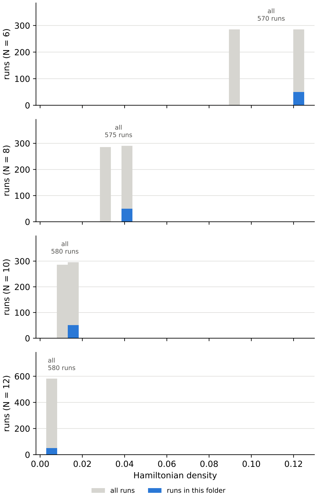
Hamiltonian density over all runs, and the cuts behind the bins lattice dimension = 2, anisotropy \delta = 100
