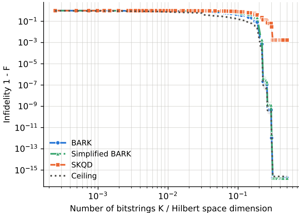
runs per point -- BARK: 114-462, Ceiling: 114-462, SKQD: 114-462, Simplified BARK: 114-462
