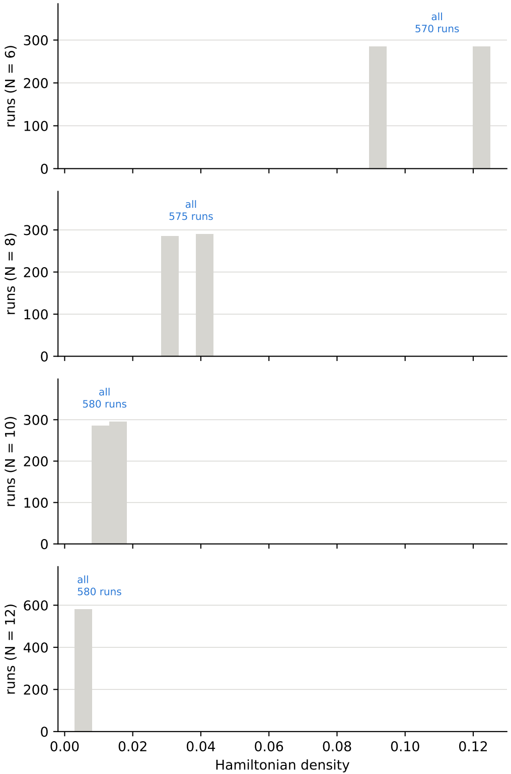
Hamiltonian density over all runs, and the cuts behind the bins Hamiltonian density = all
