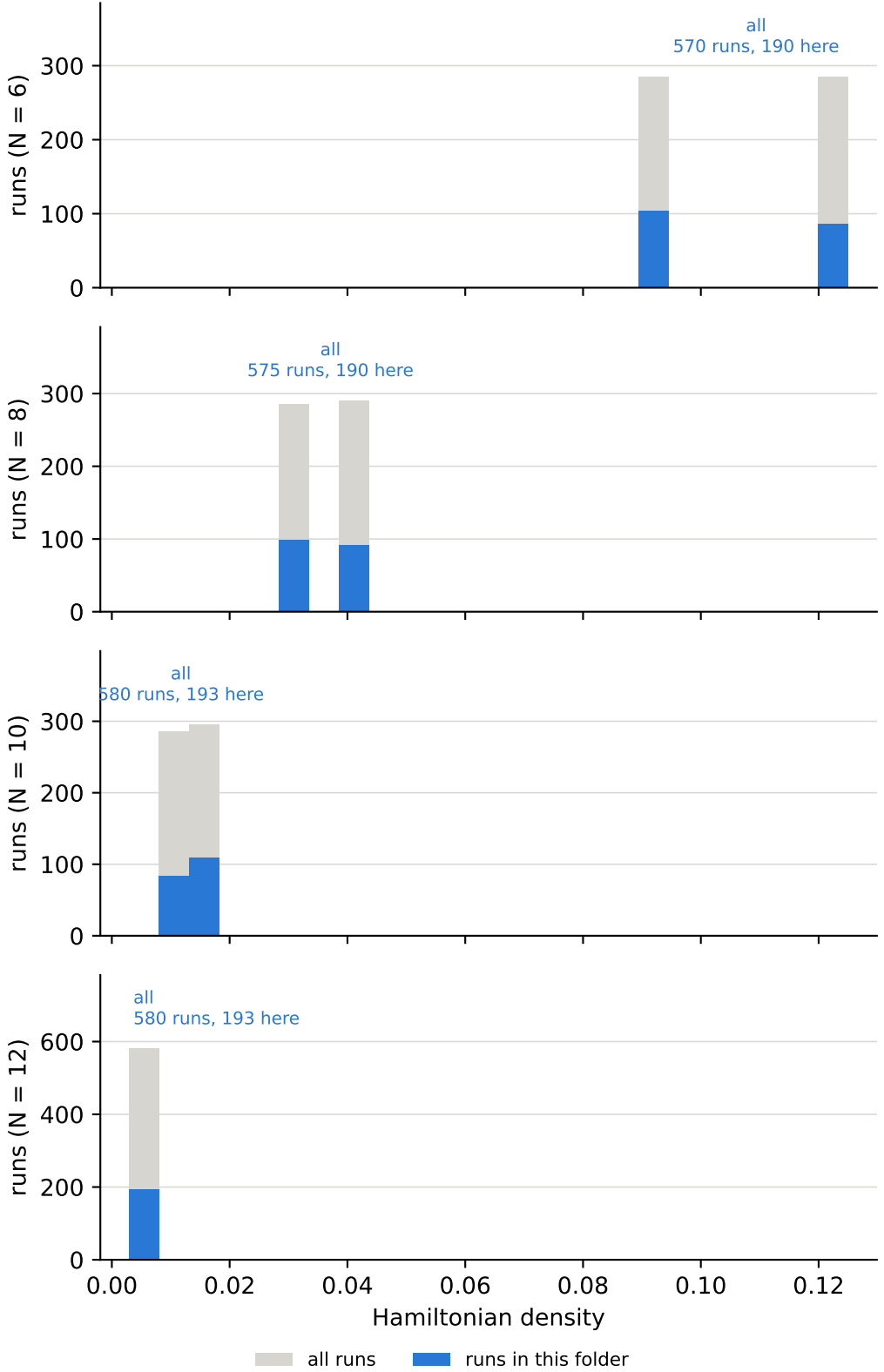
Hamiltonian density over all runs, and the cuts behind the bins Hamiltonian density = all, initial overlap = high
