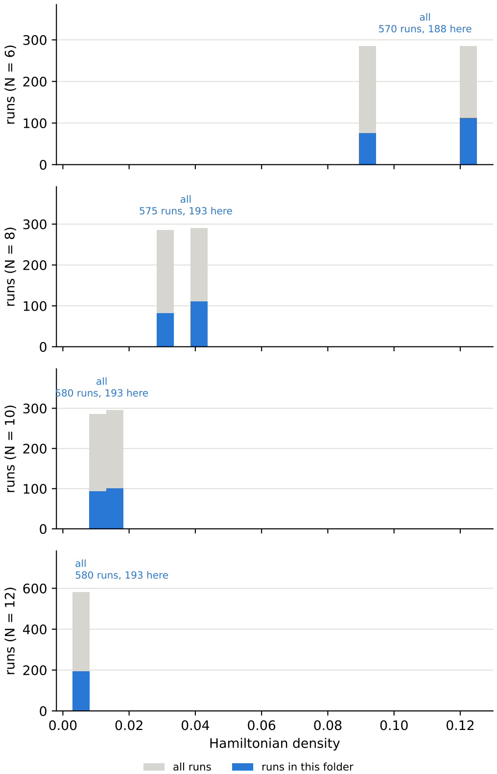
Hamiltonian density over all runs, and the cuts behind the bins Hamiltonian density = all, initial overlap = mid
