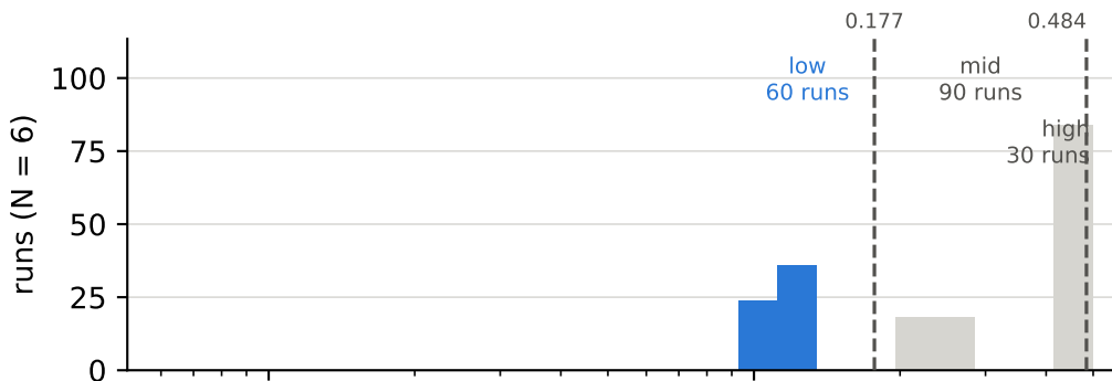
ground-state density over all runs, and the cuts behind the bins ground-state density = low
