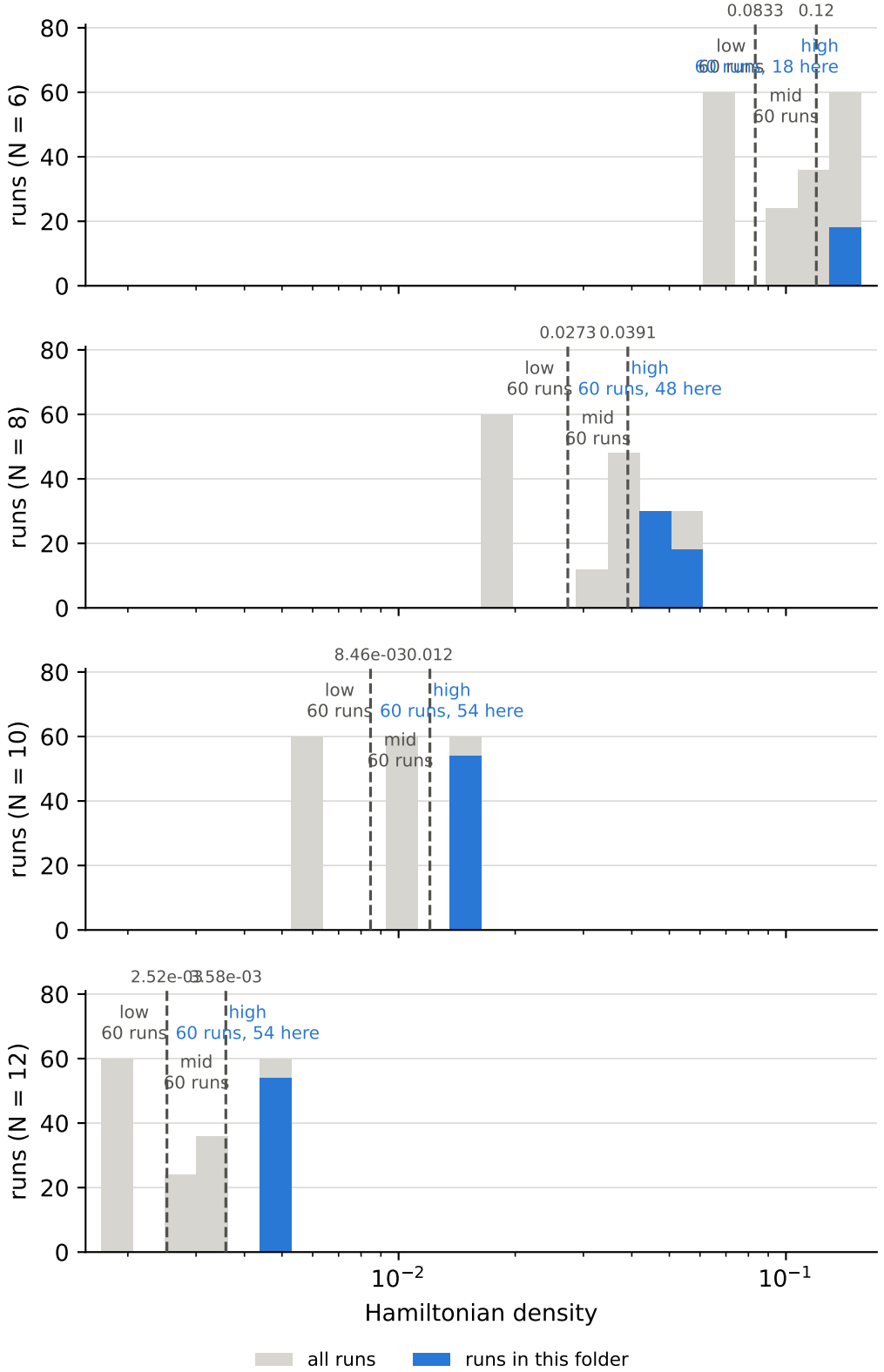
Hamiltonian density over all runs, and the cuts behind the bins ground-state density = high, Hamiltonian density = high
