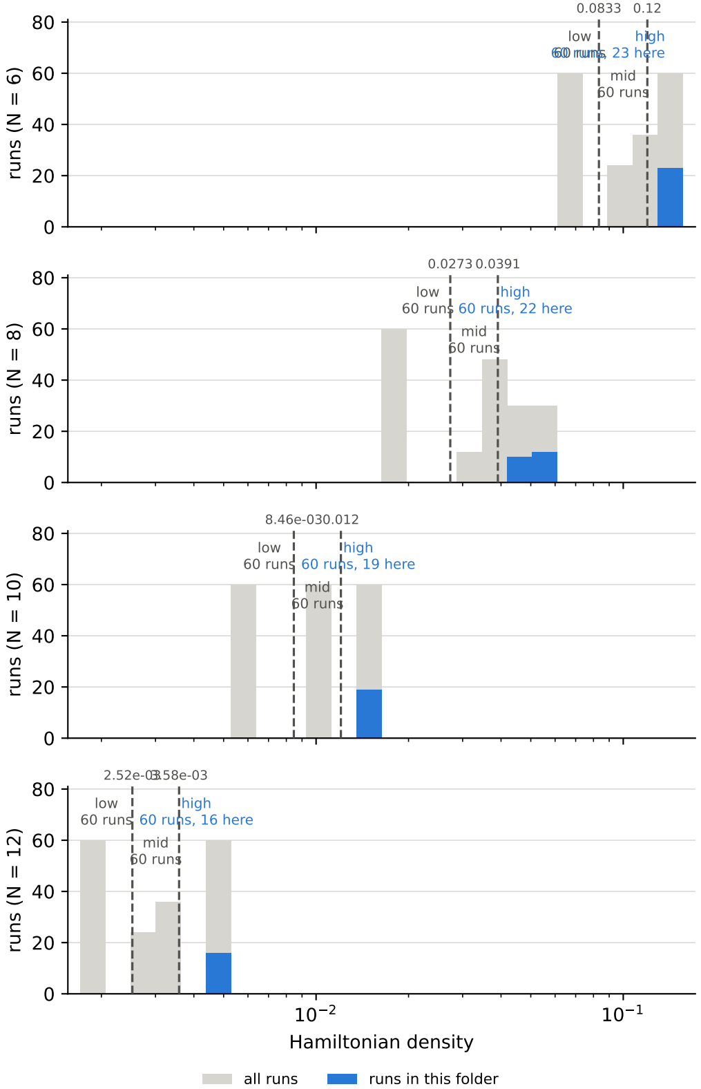
Hamiltonian density over all runs, and the cuts behind the bins Hamiltonian density = high, initial overlap = high
