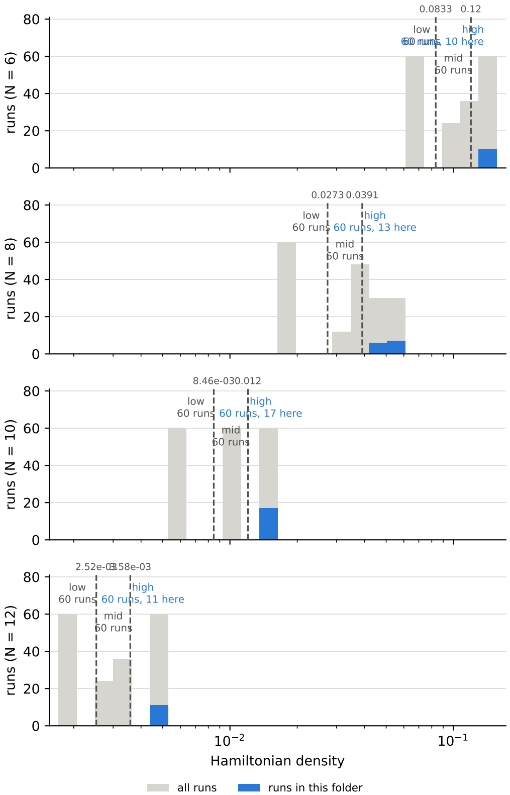
Hamiltonian density over all runs, and the cuts behind the bins Hamiltonian density = high, initial overlap = low
