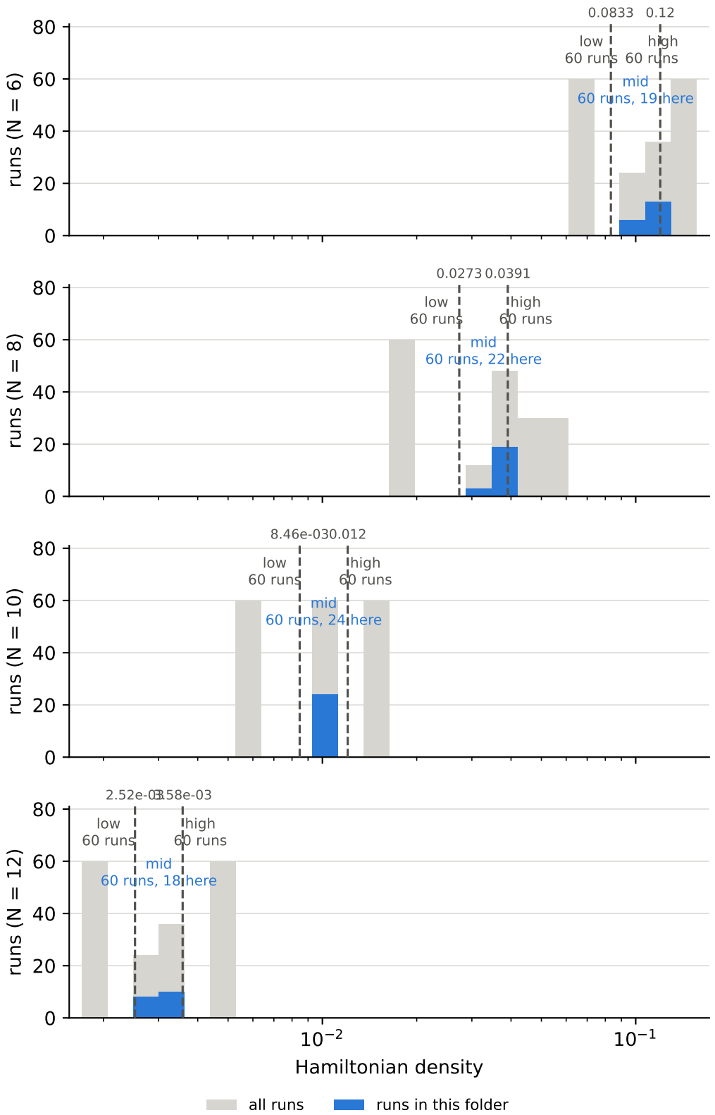
Hamiltonian density over all runs, and the cuts behind the bins Hamiltonian density = mid, initial overlap = mid
