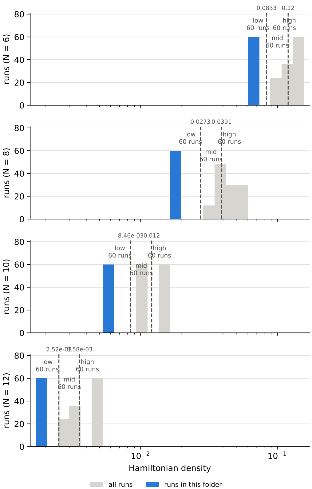
Hamiltonian density over all runs, and the cuts behind the bins max. interactions = 1
