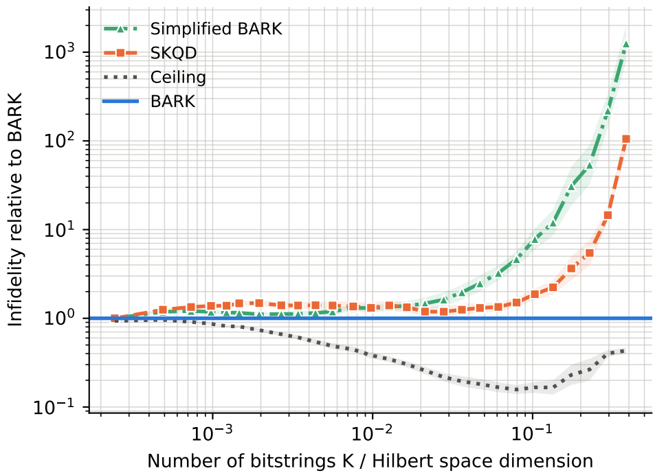
runs per point -- BARK: 15, Ceiling: 15, SKQD: 15, Simplified BARK: 15
