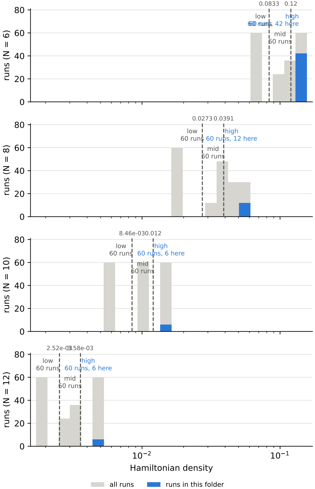
Hamiltonian density over all runs, and the cuts behind the bins ground-state density = mid, Hamiltonian density = high
