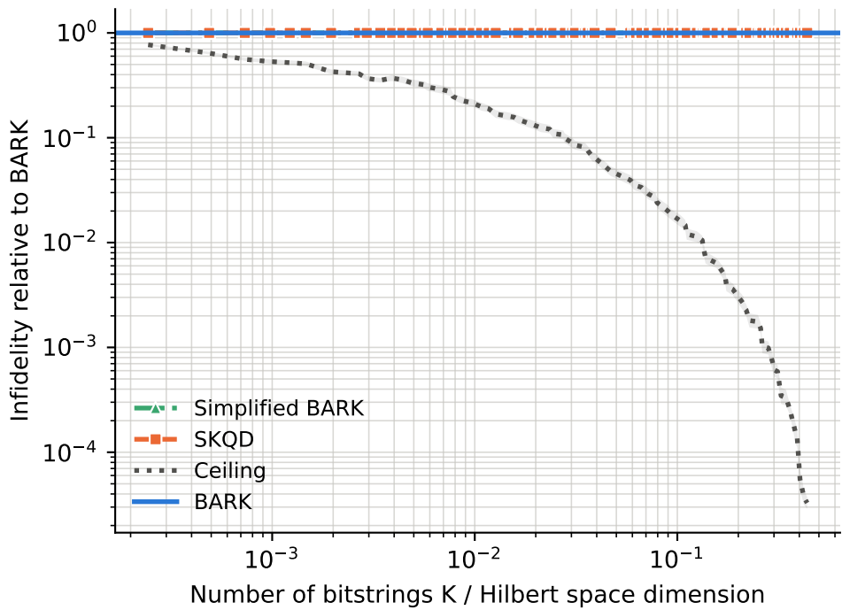
runs per point -- BARK: 8-33, Ceiling: 8-33, SKQD: 8-33, Simplified BARK: 8-33
