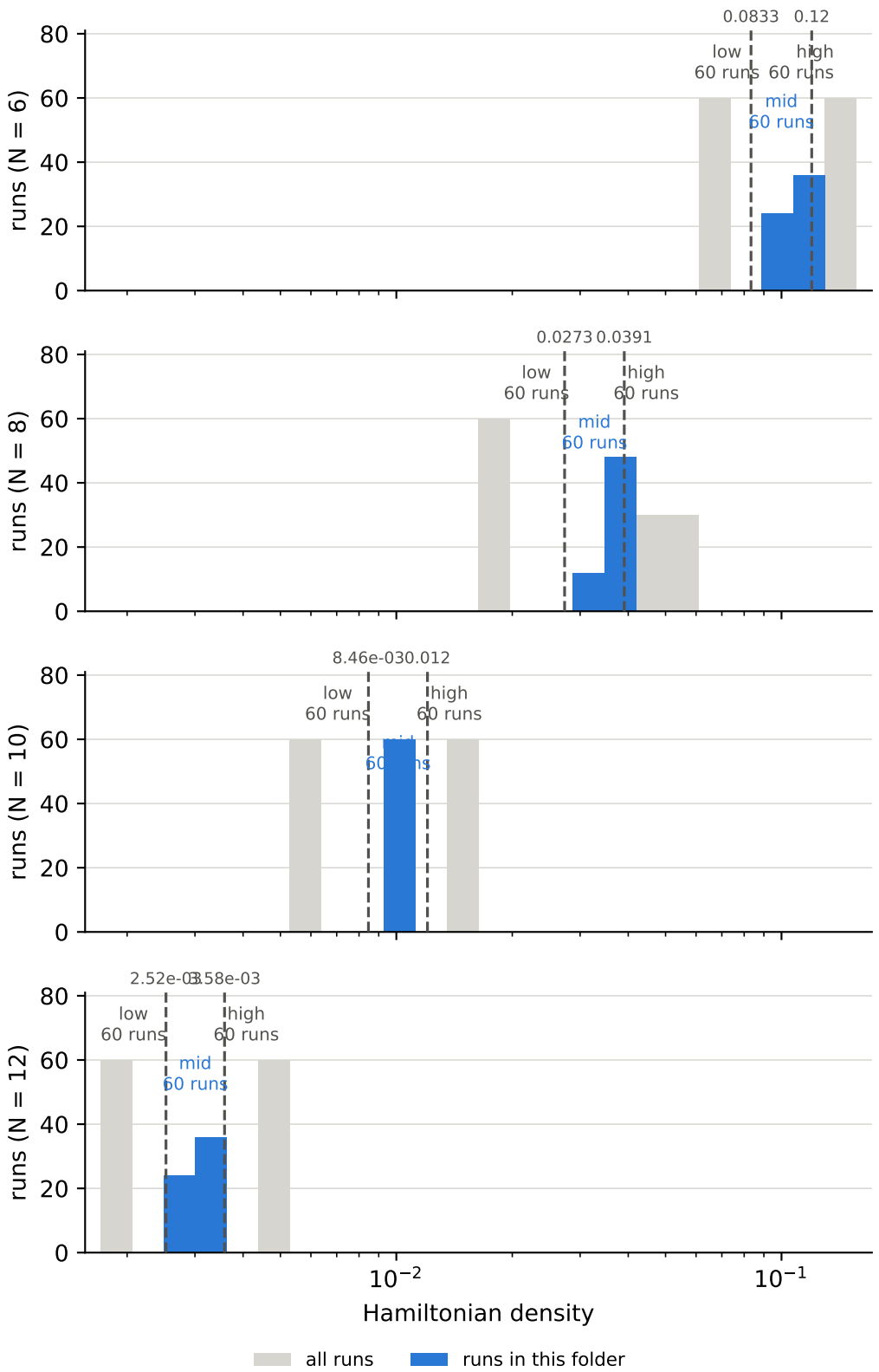
Hamiltonian density over all runs, and the cuts behind the bins Hamiltonian density = mid
