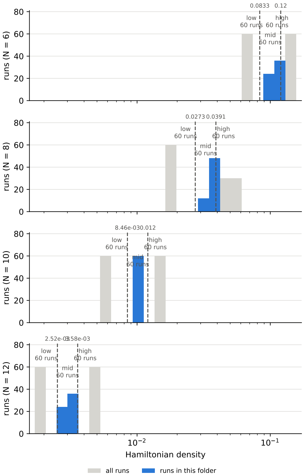
Hamiltonian density over all runs, and the cuts behind the bins max. interactions = 2
