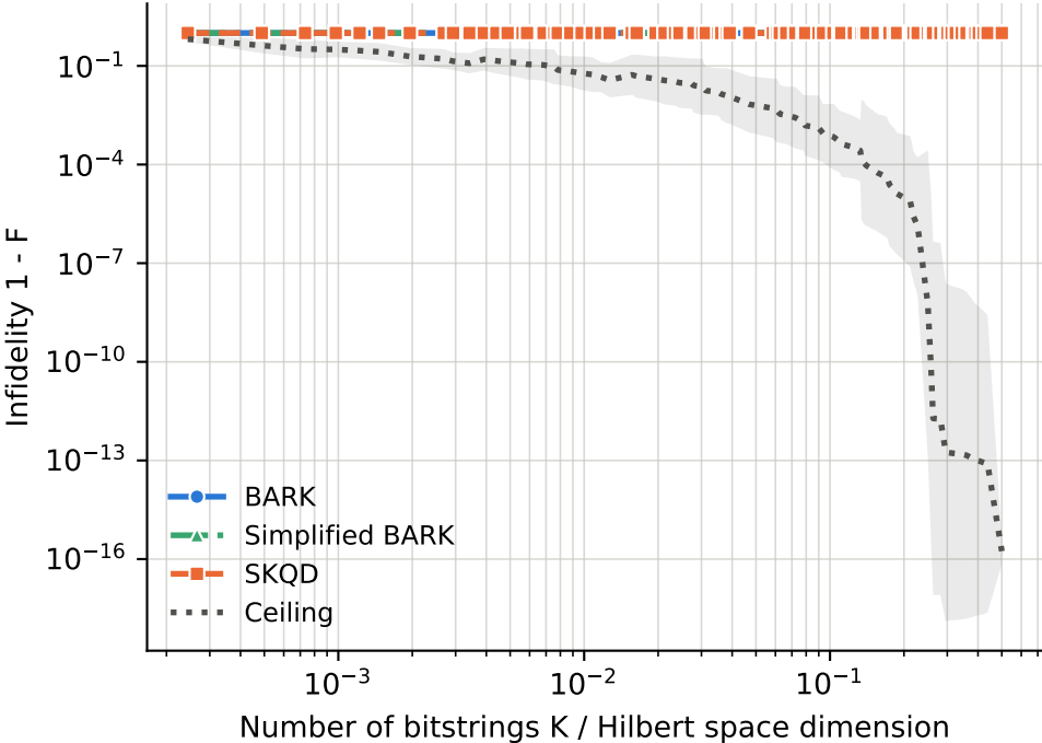
runs per point -- BARK: 16-65, Ceiling: 16-65, SKQD: 16-65, Simplified BARK: 16-65
