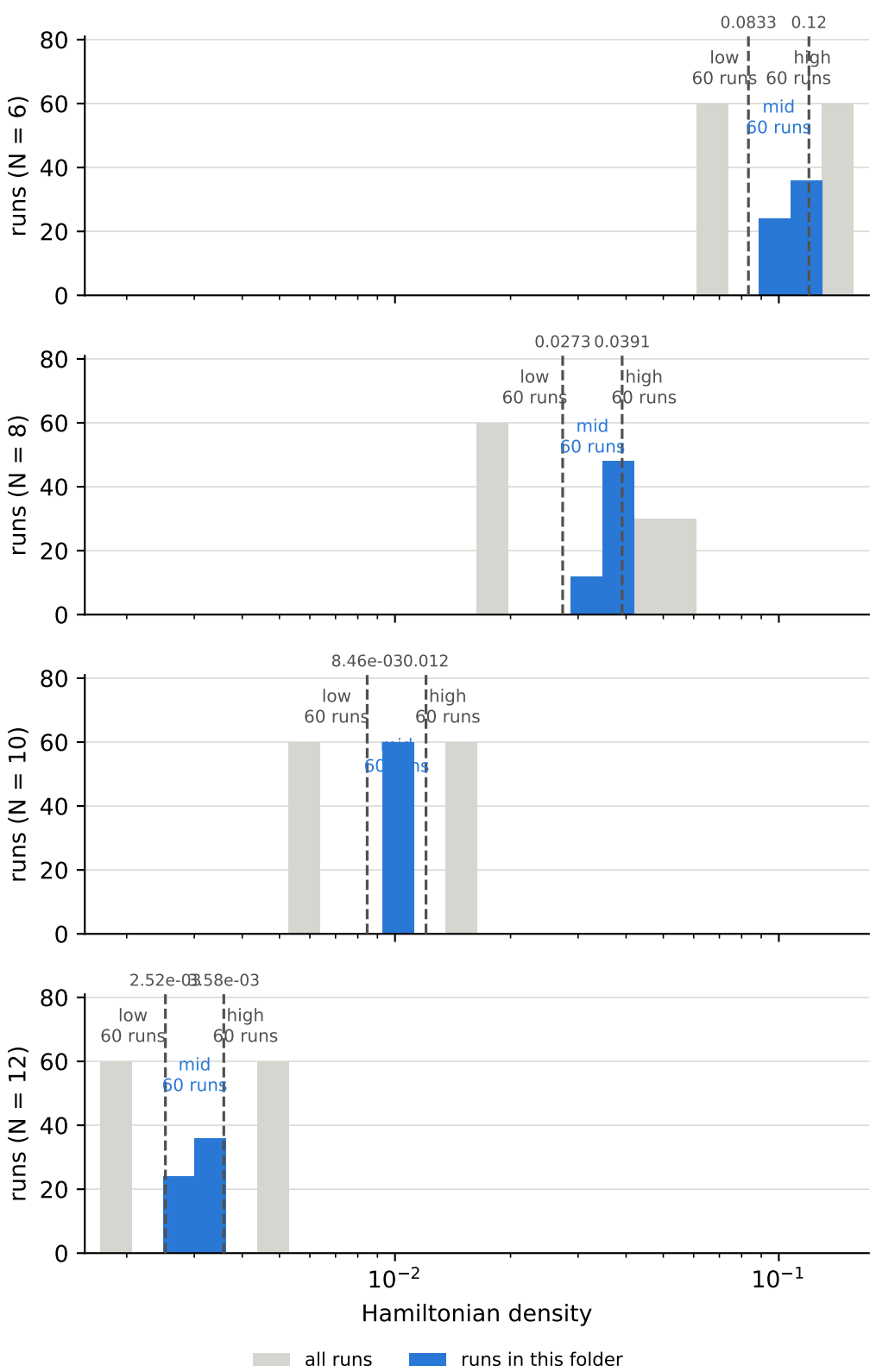
Hamiltonian density over all runs, and the cuts behind the bins max. interactions = 2, Hamiltonian density = mid
