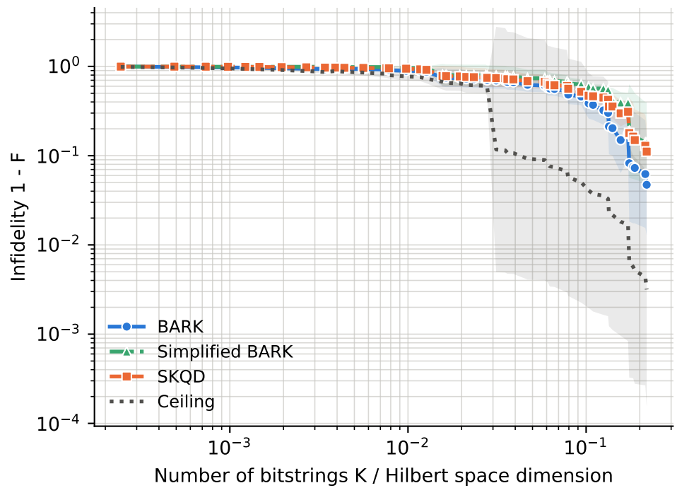
runs per point -- BARK: 8-21, Ceiling: 8-21, SKQD: 8-21, Simplified BARK: 8-21
