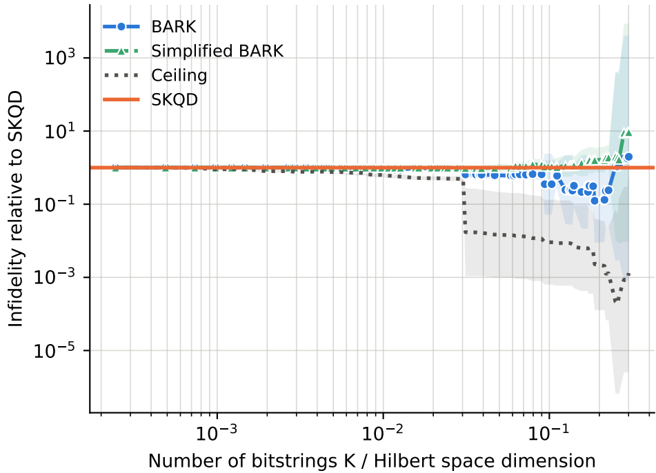
runs per point -- BARK: 1-50, Ceiling: 1-50, SKQD: 1-50, Simplified BARK: 1-50
