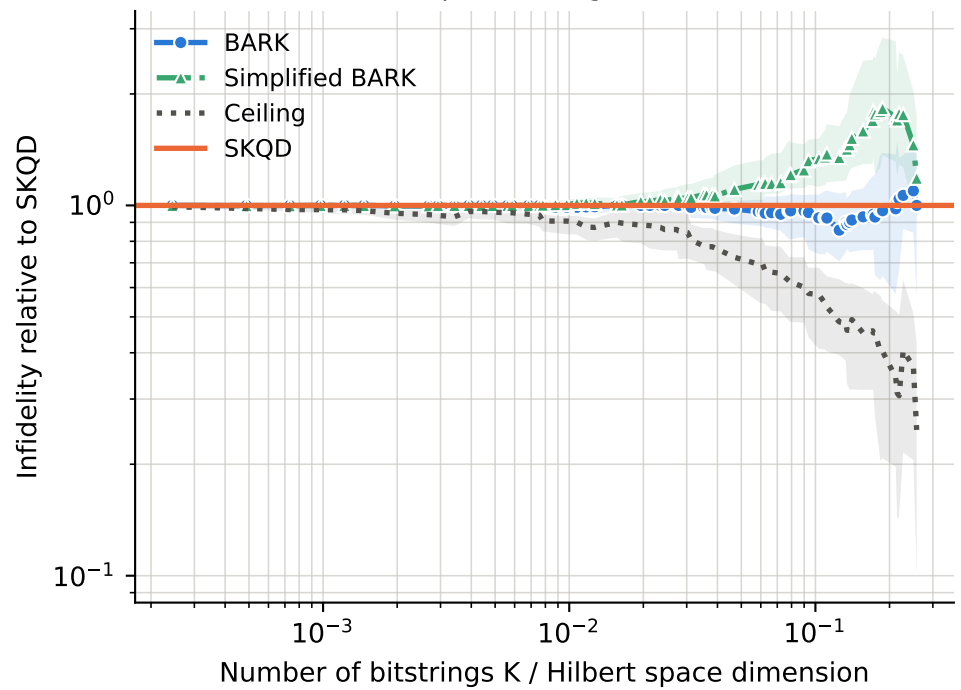
runs per point -- BARK: 13-103, Ceiling: 13-103, SKQD: 13-103, Simplified BARK: 13-103
