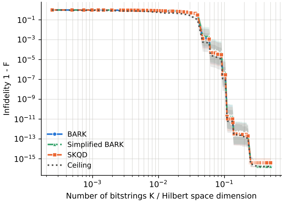
runs per point -- BARK: 4-32, Ceiling: 4-32, SKQD: 4-32, Simplified BARK: 4-32
