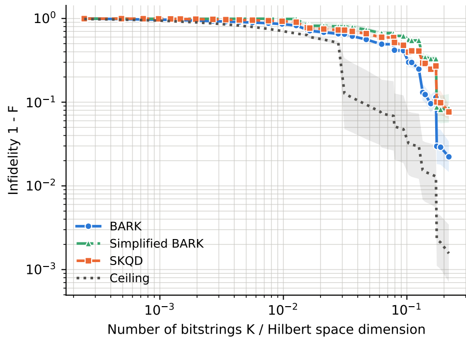
runs per point -- BARK: 6-9, Ceiling: 6-9, SKQD: 6-9, Simplified BARK: 6-9
