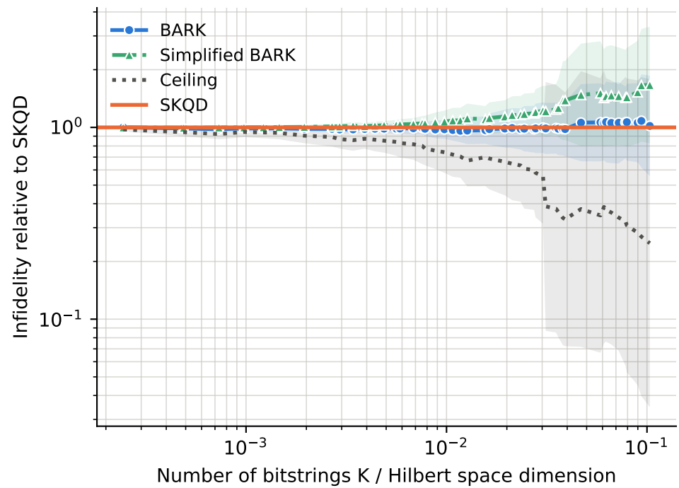
runs per point -- BARK: 9-56, Ceiling: 9-56, SKQD: 9-56, Simplified BARK: 9-56
