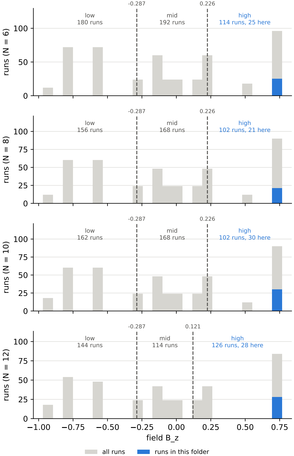
field B_z over all runs, and the cuts behind the bins coupling j = low, field B_z = high, initial overlap = high
