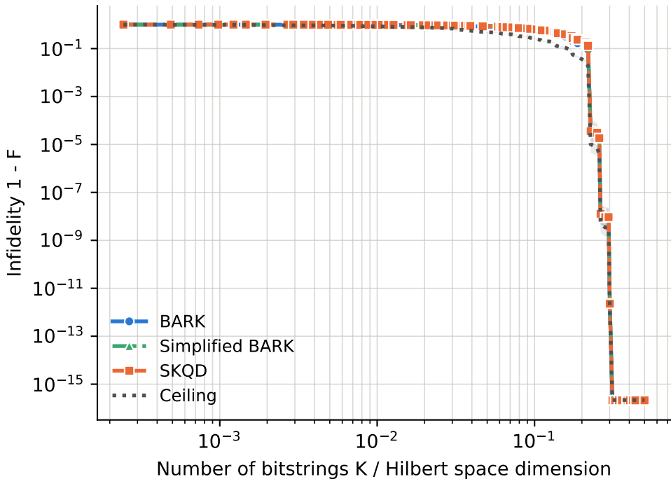
runs per point -- BARK: 72-300, Ceiling: 72-300, SKQD: 72-300, Simplified BARK: 72-300
