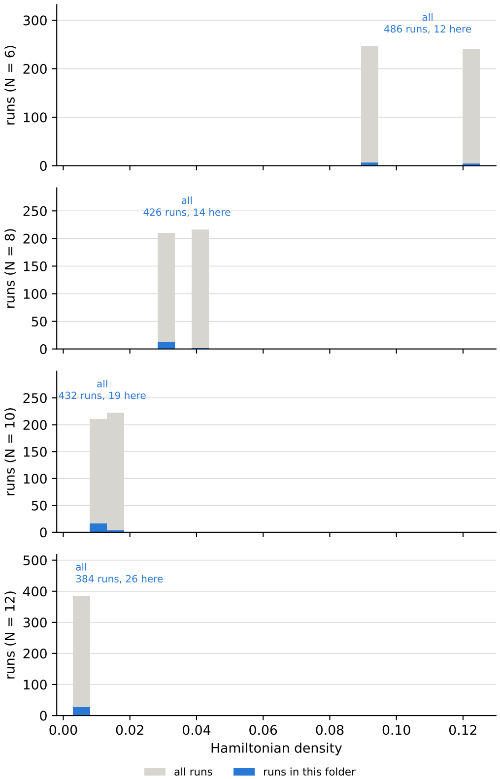
Hamiltonian density over all runs, and the cuts behind the bins coupling J = low, Hamiltonian density = all, initial overlap = low
