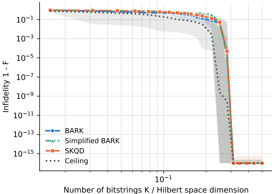
N = 6 (band: interquartile range, line: median)
