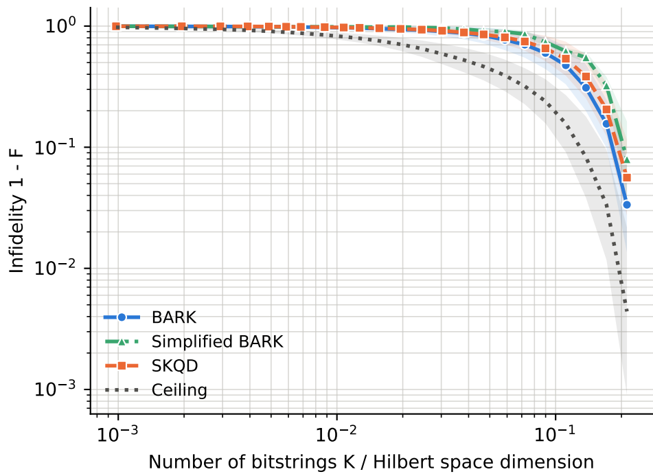
runs per point -- BARK: 66, Ceiling: 66, SKQD: 66, Simplified BARK: 66
